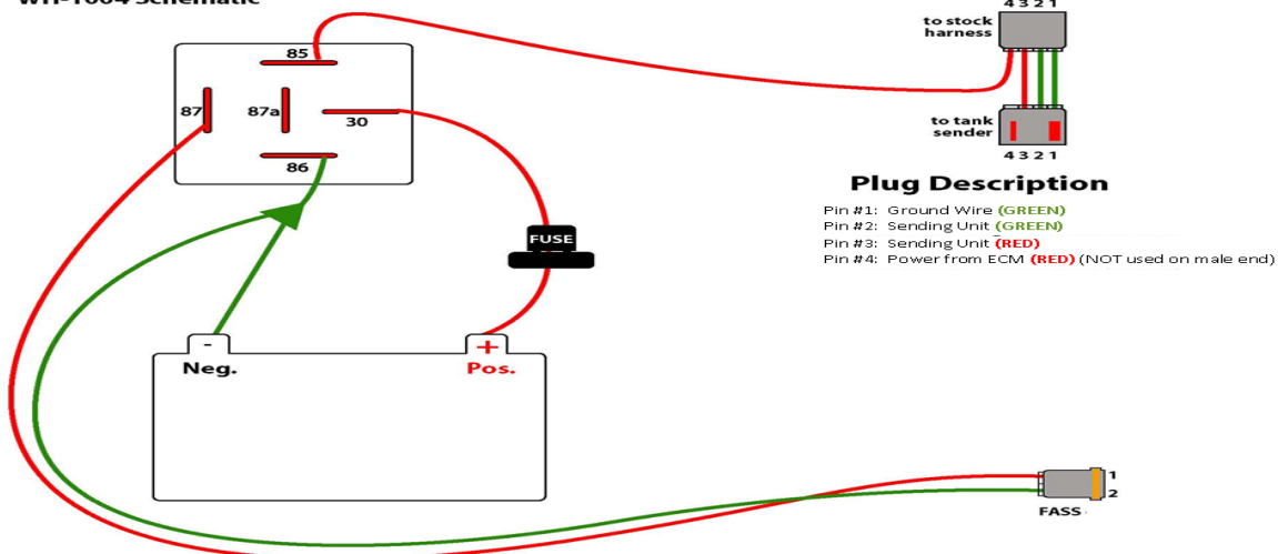
FASS Wiring Harness WH-1004 Schematic
