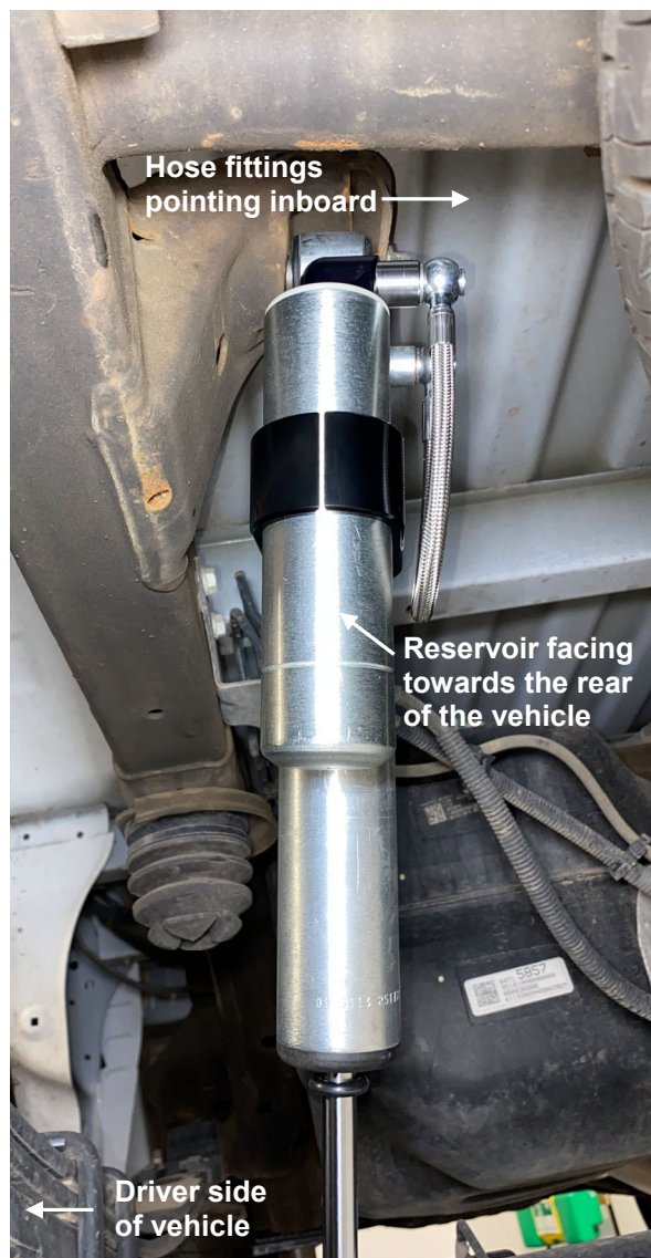
Figure 5. Driver Side (Rear View)
